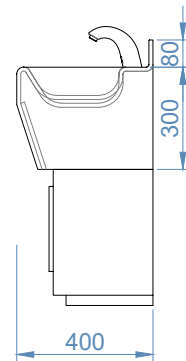
Latherwash 2D Curve 1800 - Side View
