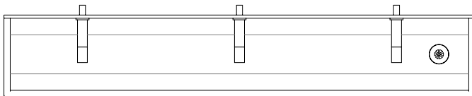
Latherwash 2W Curve 1800 - Plan View
