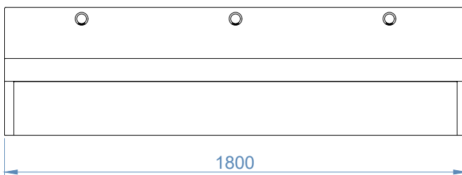
Latherwash 2W Curve 1800 - Front View
