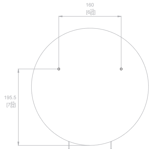
Fixing Locations
