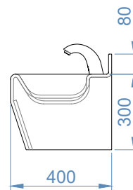
Latherwash 2D Curve 1800 - Side View
