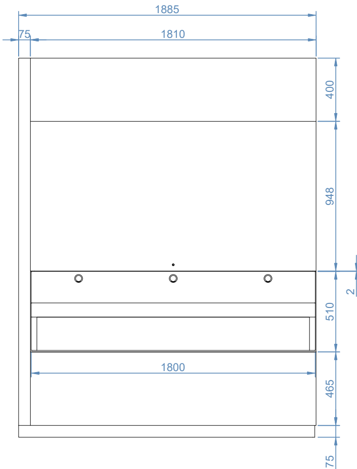
Latherwash Wall 1800 - Front View
