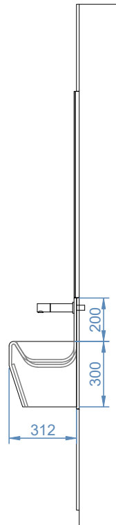
Latherwash Wall 1800 - Side View
